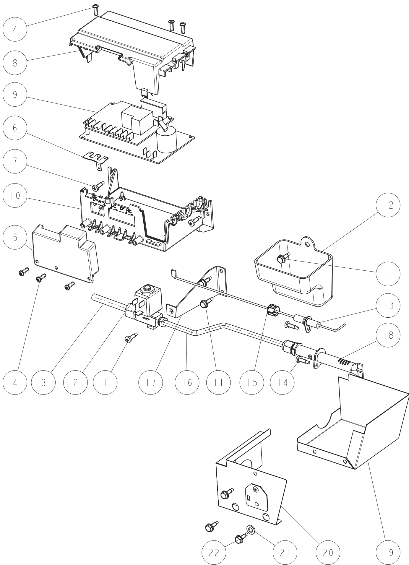
LE-439 EXPLODED
