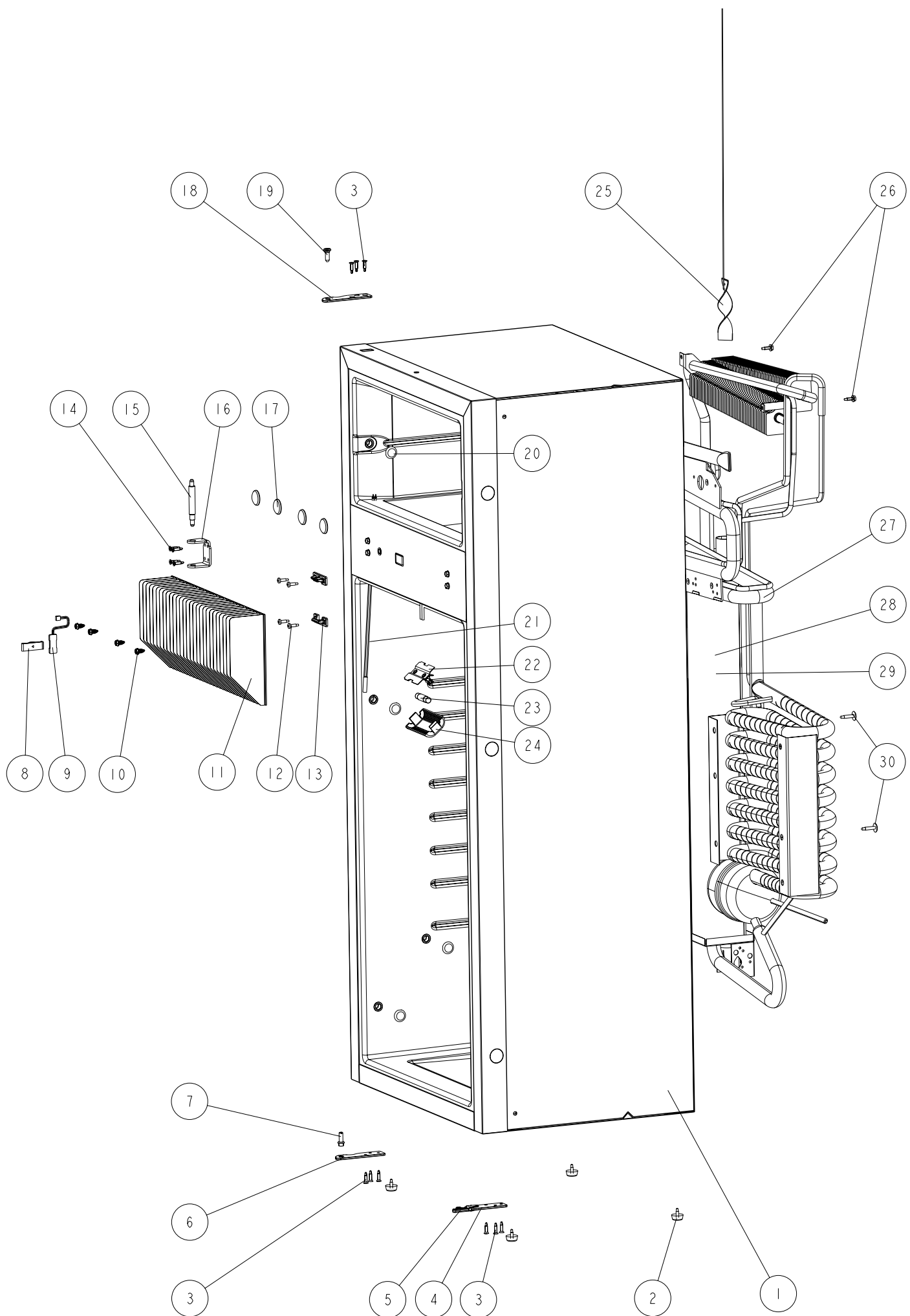
LE232-EXPLODED
