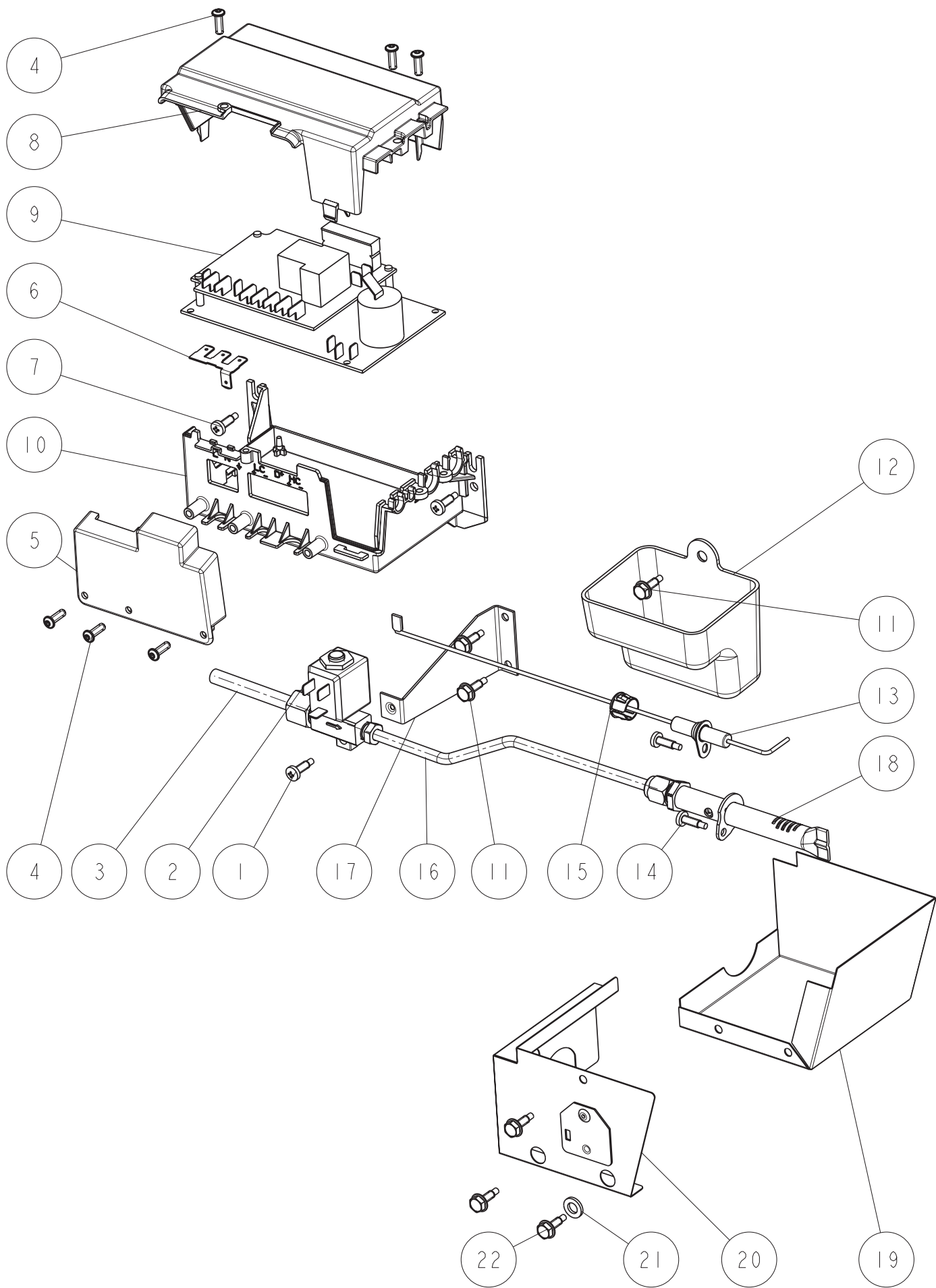
LE-439 EXPLODED
